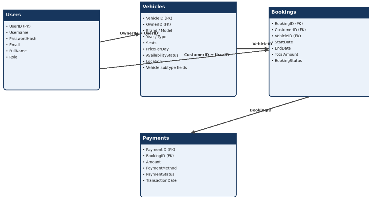
Figure 1: Entity-Relationship Diagram of the Car Rental Management System
